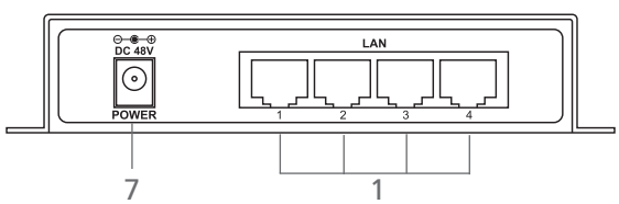
Figure 2-2. Back panel.
